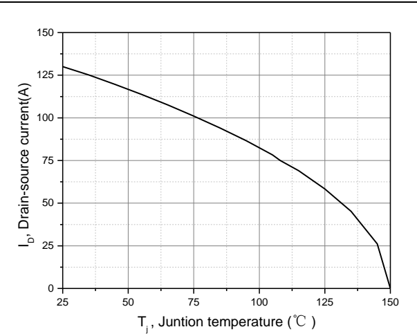
Figure 8. Drain current
