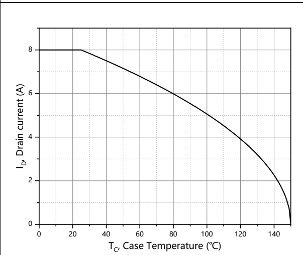
Figure 10. Drain current
